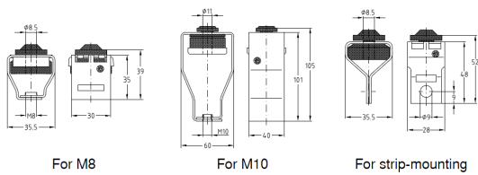
For M8
